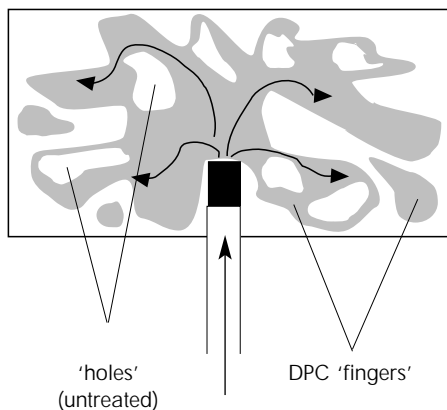
Figure 7: Fingering effect of pressure injected DPC fluid
