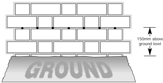
Figure 9: Drilling pattern for Double Flemish Bond.
