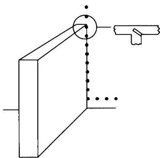
Vertical DPC to isolate abutting walls, etc.
