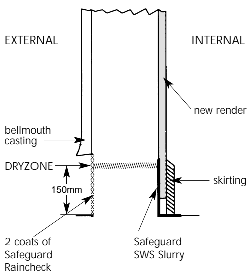
Figure 17: Suggested finishing work
