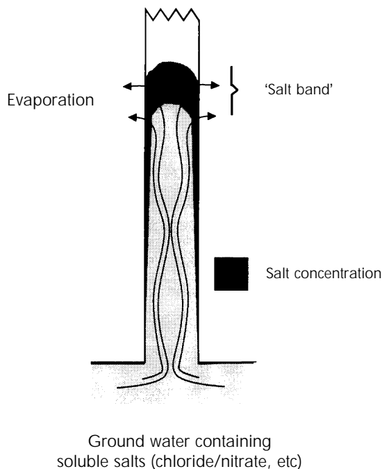
Figure 2: A rising damp complex
