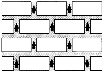
Figure 1: Water rising through mortar beds
